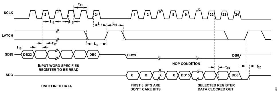
Figure 3. Readback Mode Timing Diagram
