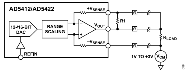
Figure 67. Voltage Output
