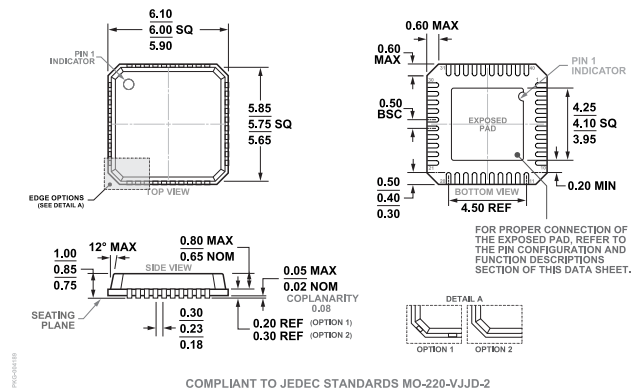
Figure 85. 40-Lead Lead Frame Chip Scale Package [LFCSP] (CP-40-1) 6 mm × 6 mm Body and 0.85 mm Package Height Dimensions shown in millimeters
