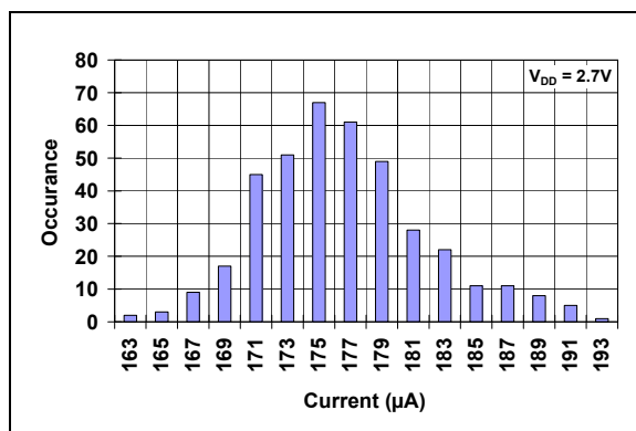
FIGURE 2-13: I_{DD} Histogram.
