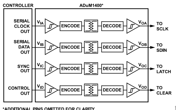
Figure 52. Isolated Interface
