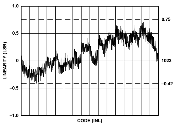
Figure 18. Typical Linearity
